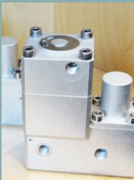
Dual stage Hydrogen regulator Inlet Pressure: 400 bar Outlet Pressure: 0 - 5 bar +/- 100 mbar
